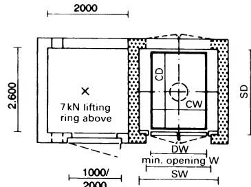
② Plan view of shaft with lift motor room
